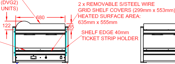
FRONT VIEW (CUSTOMER SIDE)
