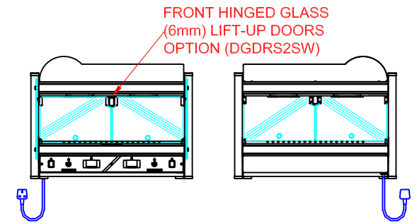
FRONT VIEW (CUSTOMER SIDE) c/w FRONT DOOR OPTION
