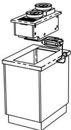
FRONT ISOMETRIC (CUSTOMER SIDE)
