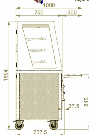
Glide Amb. Multideck - Doors (Self Help/ Ass. Serve) + Tray Rail
