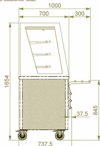
Glide Amb. Multideck - Fixed Back (Self Help) + Tray Rail
