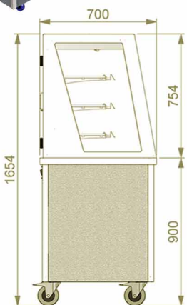
Glide Amb. Multideck - Doors (Self Help/ Ass. Serve)
