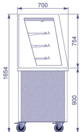
Glide Cold Multideck - Fixed Back (Self Help)
