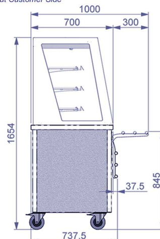
Glide Cold Multideck - Fixed Back (Self Help) + Tray Rail
