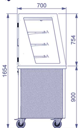
Glide Cold Multideck - Doors (Self Help/ Ass. Serve)
