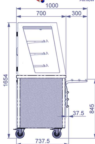
Glide Cold Multideck - Doors (Self Help/ Ass. Serve) + Tray Rail
