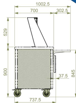
Glide Wall Sited Sanitising Unit & Tray Slide
