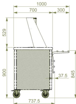
Glide Wall Sited Sanitising Unit & Tray Rail
