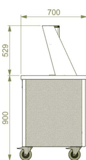
Glide Wall Sited Sanitising Unit
