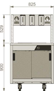
Glide Wall Sited Sanitising Unit
